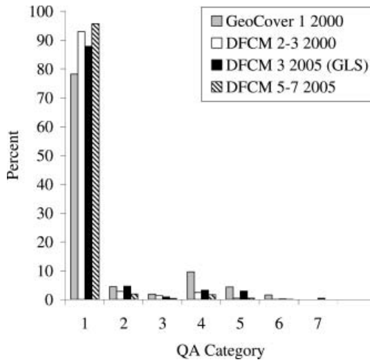
Figure 2. Histograms of the percentage of pixels in the four Landsat epochal mosaics for each QA value. QA values in descending order of quality are: 1, no cloud/haze or shadow (i.e. best quality); 2, low likelihood of cloud/haze; 3, low likelihood of shadow; 4, adjacent to high likelihood cloud/haze or shadow; 5, high likelihood of cloud/haze; 6, high likelihood of shadow; 7, missing due to SLC-off gaps. The four Landsat epochal mosaics are labelled in the key as method, number of Landsat acquisitions used per path/row, and epoch period. See text for further details.
